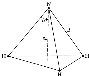
10.16 Schematic diagram of the ammonia molecule.
